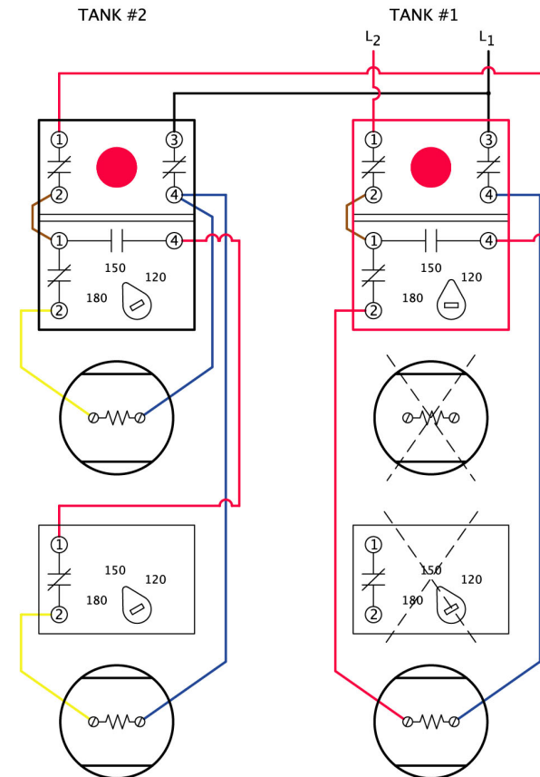
STORED WATER THERMOSTAT WIRING DUAL TANK SYSTEM
